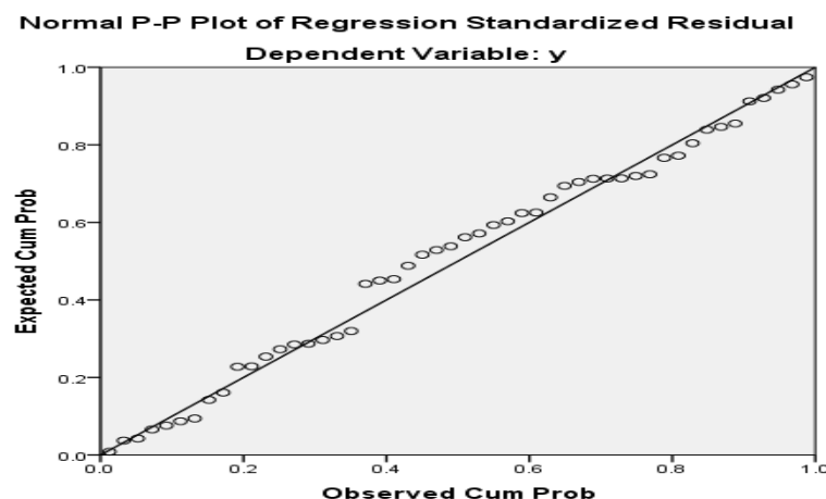
Gambar 1. Grafik Normalitas Probabilitiy Plot
