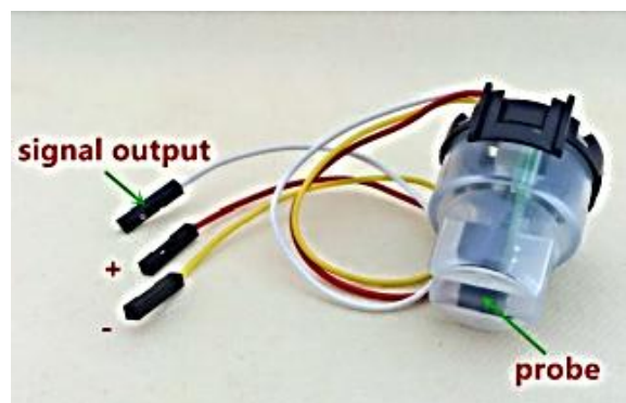
Gambar 12 Turbidity sensor
